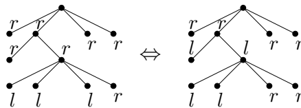
Figure 4: The involution \phi
