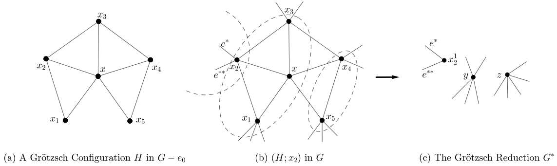
Figure 1: A Grötzsch Configuration and some related graphs.
