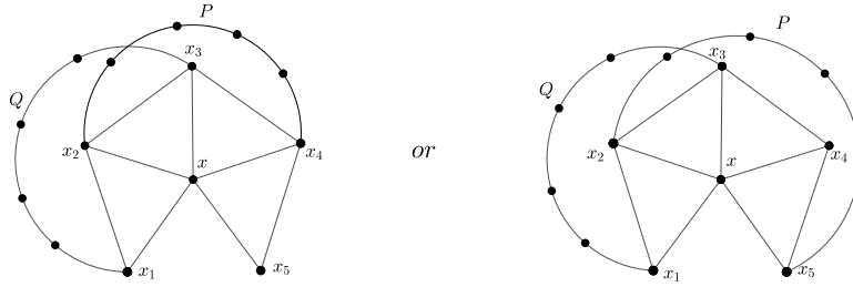
Figure 5: The paths P and Q in G - e_0 .
