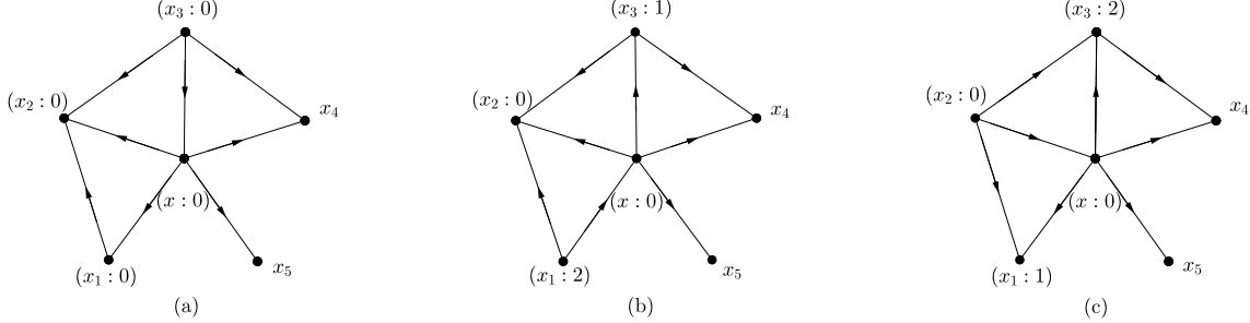
Figure 6: Some orientations of the graph H - x_4x_5 in Claim VII.
