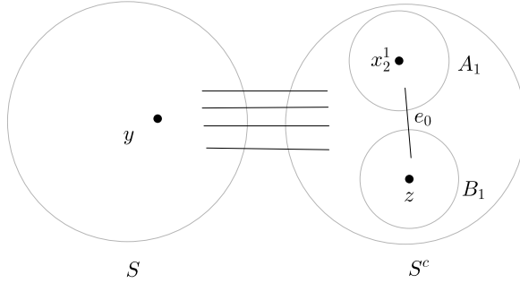
Figure 3: The edge-cut [S, S^c]_{G^*} of G^* .
