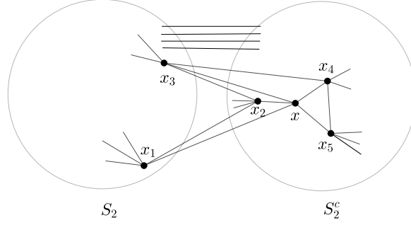
Figure 4: The edge-cut [S_2, S_2^c]_G of G .
