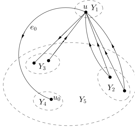
Figure 2: A partition \{Y_1, Y_2, Y_3, Y_4, Y_5\} of V(G) .
