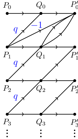
Figure 3.1: The planar network \mathcal{L}^B
