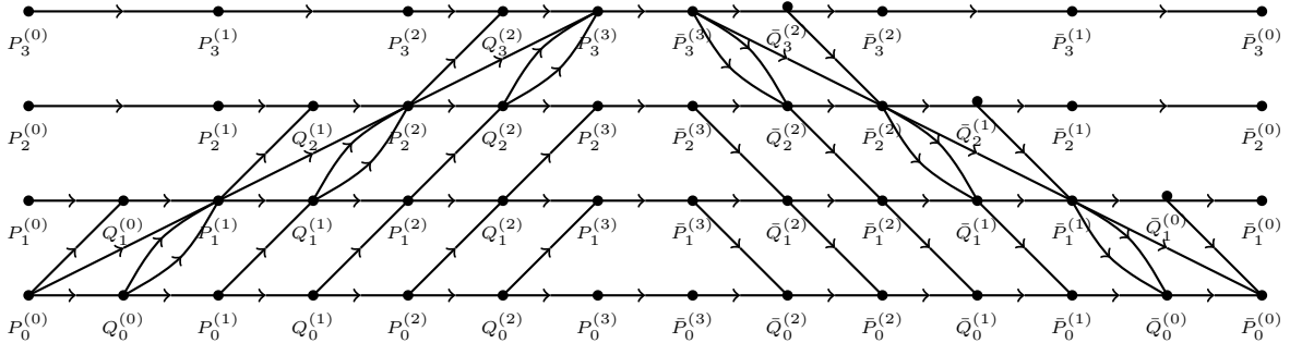
Figure 4.3: Digraph D^{H_3}
