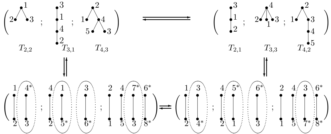
FIGURE 2. A bijection on labelled plane forest.
