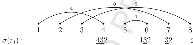
Fig. 3. The major index for partition 14-27-38-56 is 4.
