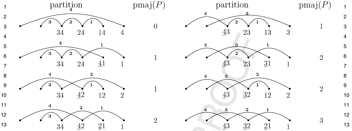
Fig. 5. \text{pmaj}(P) for P \in P_6(\{1, 2\}, \{5, 6\}) .
