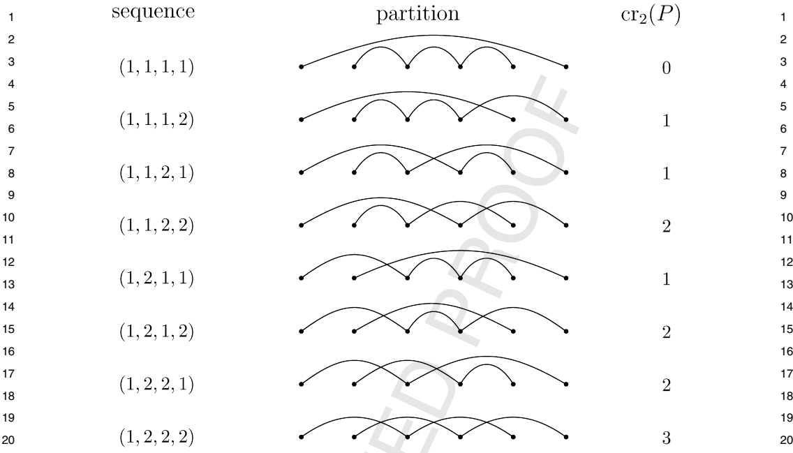
Fig. 4. cr_2(P) for P \in P_6(\{1, 2\}, \{5, 6\}) .
