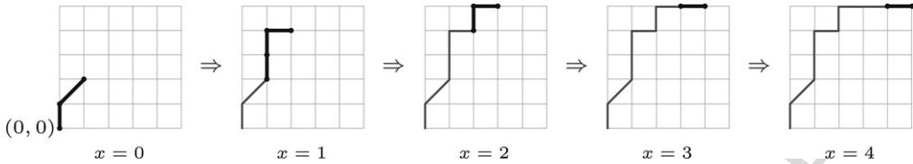
Fig. 3. The steps of \phi that yield the corresponding Schröder path.
