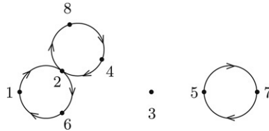
Fig. 7. The cycle representation of the linked cycle \pi = (126)(284)(3)(57) .
