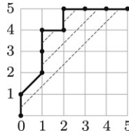
Fig. 2. There are four tunnels in the Schröder path.
