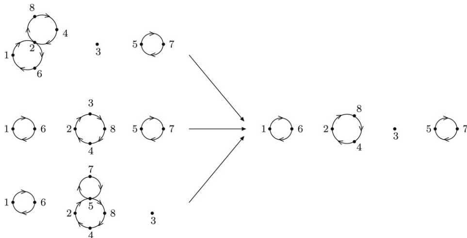
Fig. 8. The operation \tau on three linked cycles with 3 components all gives the same linked cycle with 4 components.
