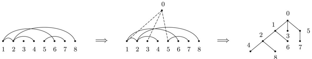
Fig. 5. A linked partition and the corresponding increasing tree.
