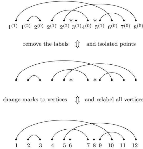
Fig. 9. The procedure from a linked cycle to a partition.
