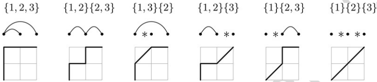
Fig. 4. The elements of NCL(3) and their corresponding Schröder paths.
