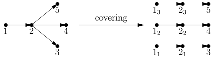
Figure 3: The covering of a rooted tree with line-graphs
