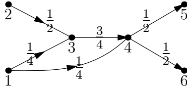
Figure 1: A flow in an acyclic digraph
