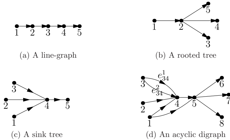
Figure 2: A line-graph, a rooted tree, a sink tree and an acyclic digraph
