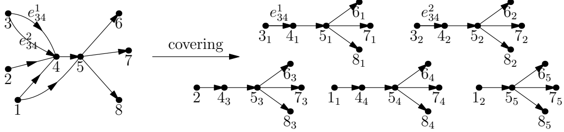
Figure 4: A covering of an acyclic digraph with rooted trees
