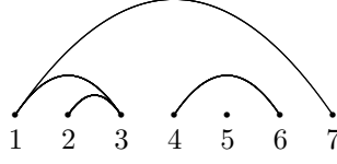
Figure 4.2: A zigzag stack on [7] .
