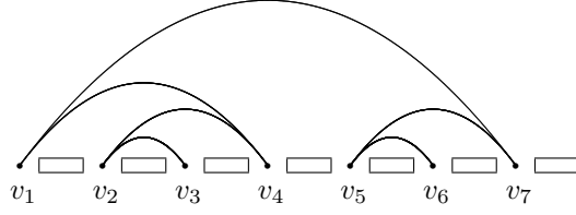
Figure 2.1: Decomposition of a zigzag stack.
