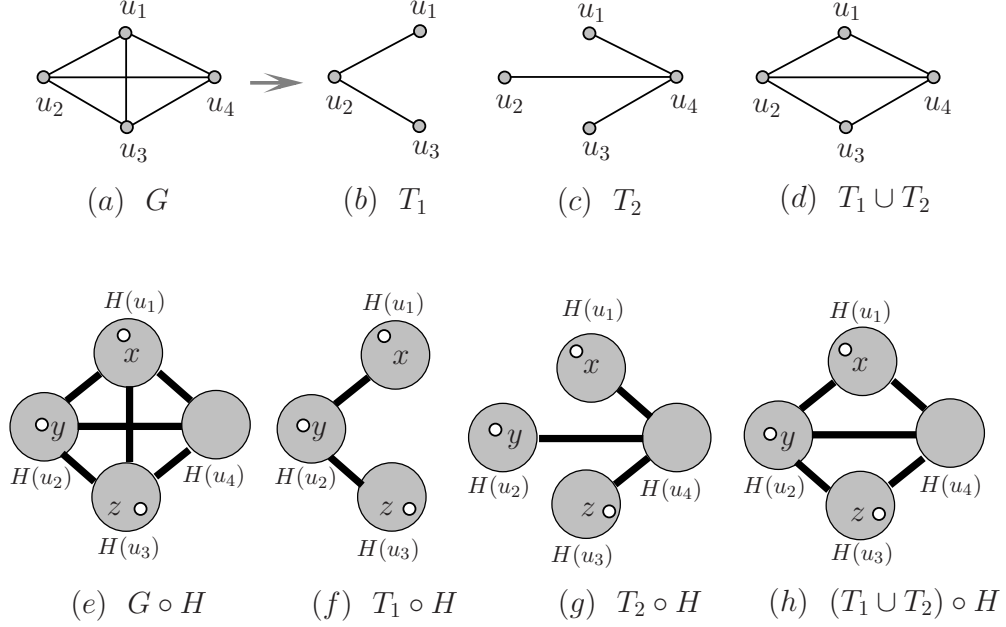
Figure 2.1 An example for G \circ H .
