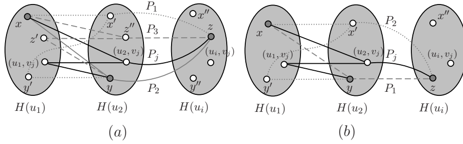
Figure 2.5 Graphs for Case 2 of Lemma 2.6.
