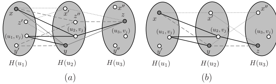
Figure 2.4 Graphs for Case 1 of Lemma 2.6.
