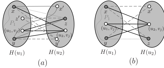
Figure 2.3 Graphs for Lemma 2.5.
