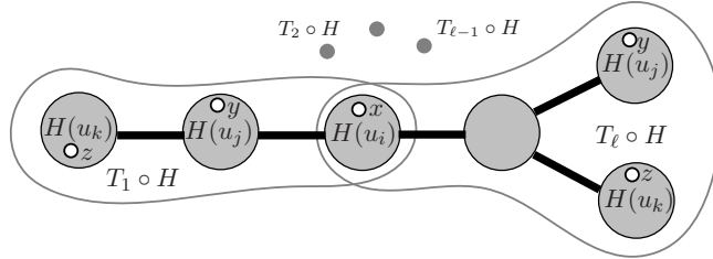
Figure 2.2 The structure of (\bigcup_{i=1}^k T_i) \circ H = \bigcup_{i=1}^k (T_i \circ H) .
