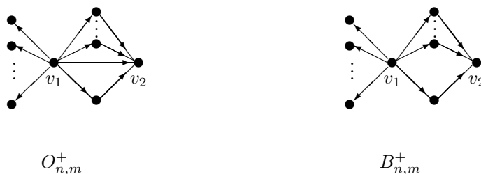
Fig. 1.1. Oriented graphs O_{n,m}^+ and B_{n,m}^+ .
